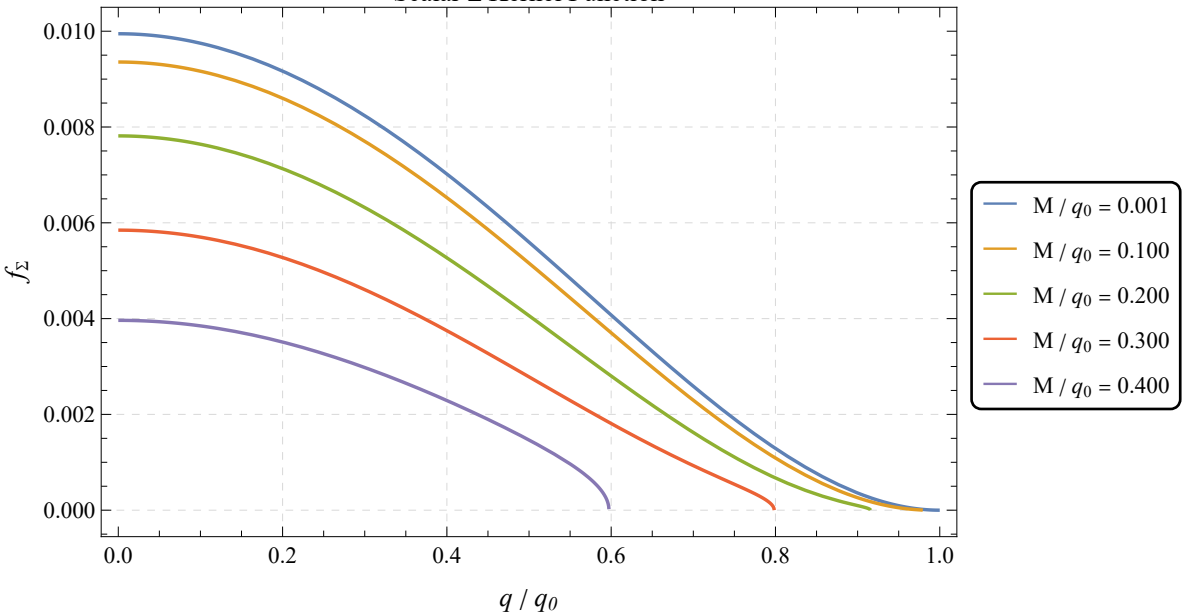
Scalar \Sigma Kernel Function
